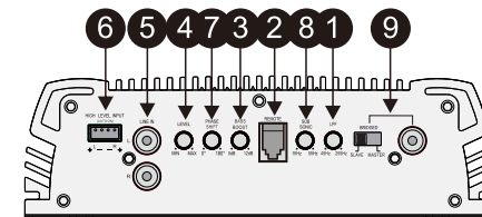
QM 500.1 FRONT PANEL
